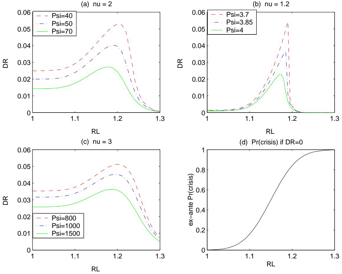
Figure 3: Continuous set of actions for the government
