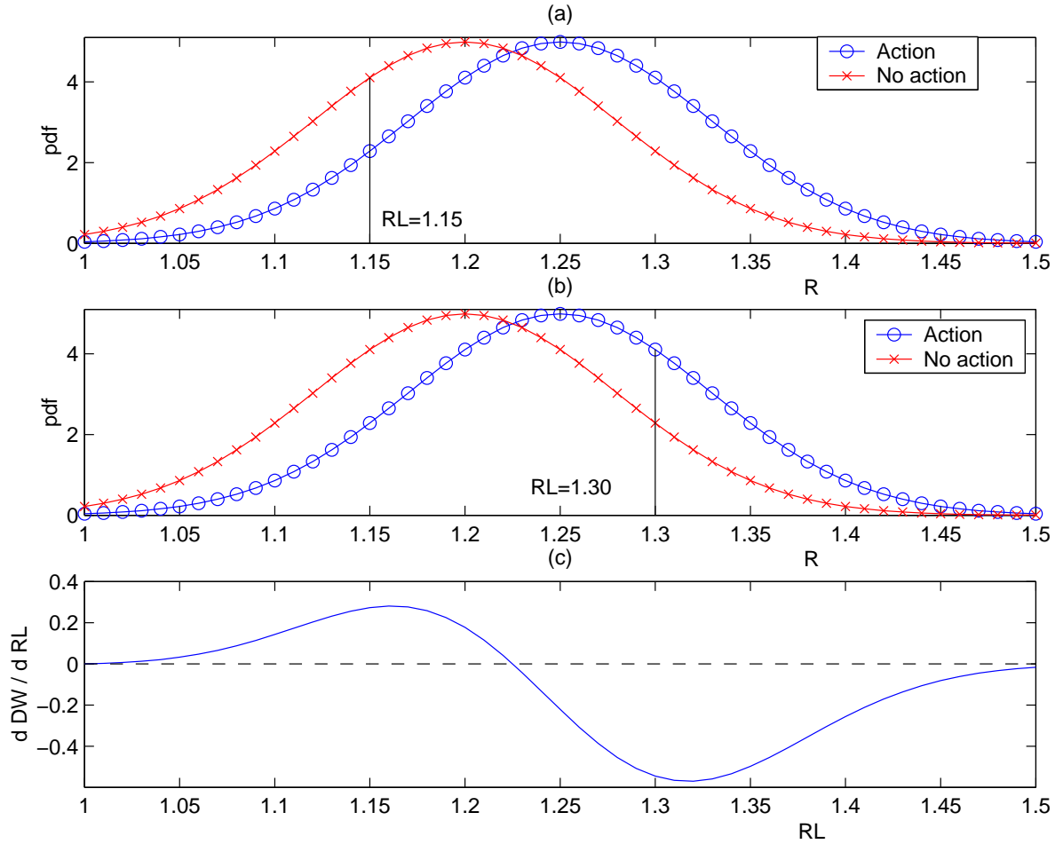
Figure 1: Government's decision: \Delta W and \bar{R}_L
