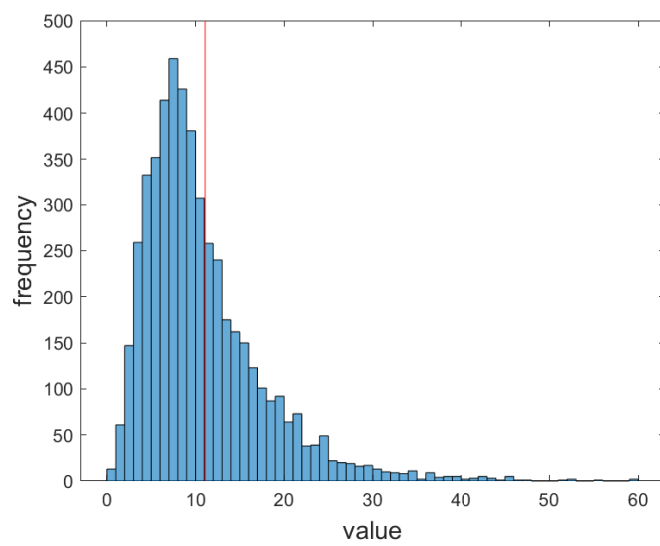
Figure 5: Mertens and Montiel Olea (2018) : Block Bootstrap Distribution of the F-statistic Notes: Red line shows value of 11.09 in the data.
