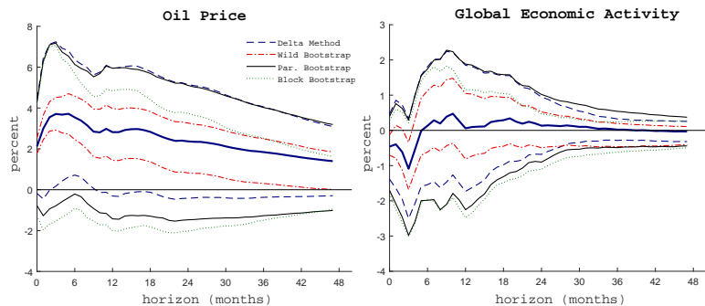
Figure 4: Impulses and 68% Standard Percentile Intervals in Selected Applications of Proxy SVARs.
