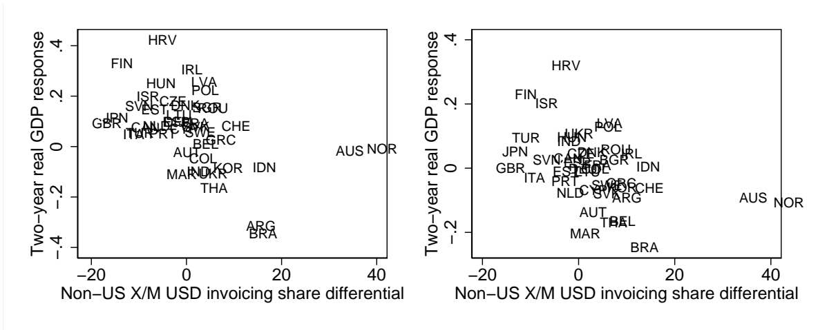
Figure 9: Relationship between spillovers from a positive US demand shock and non-US export/import US dollar invoicing share differential
