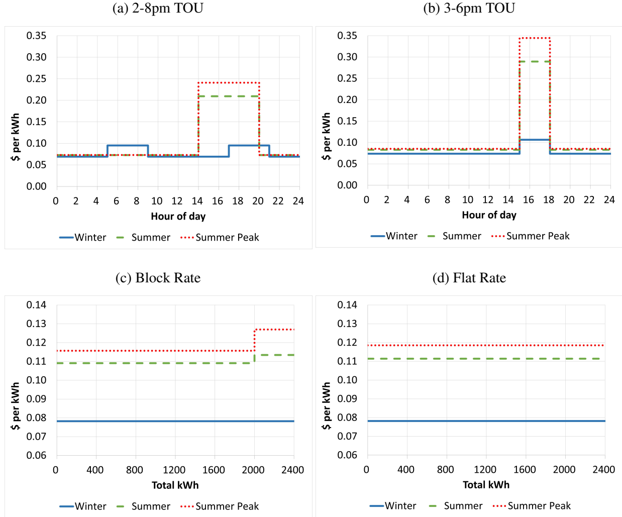
Figure 1: Plan-specific Prices by Hour of Day and Season
