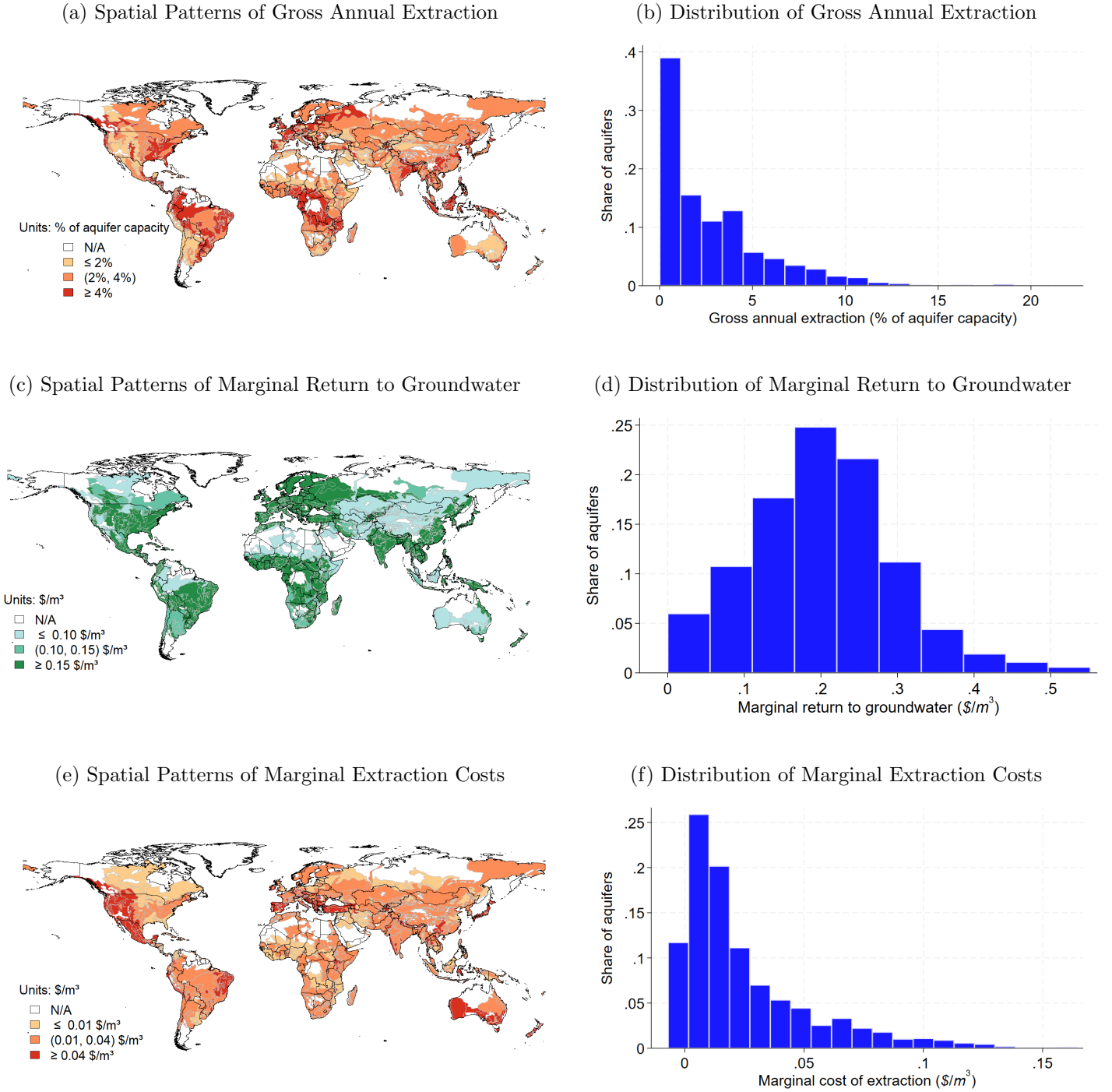
Figure 2: Aquifer Characteristics
