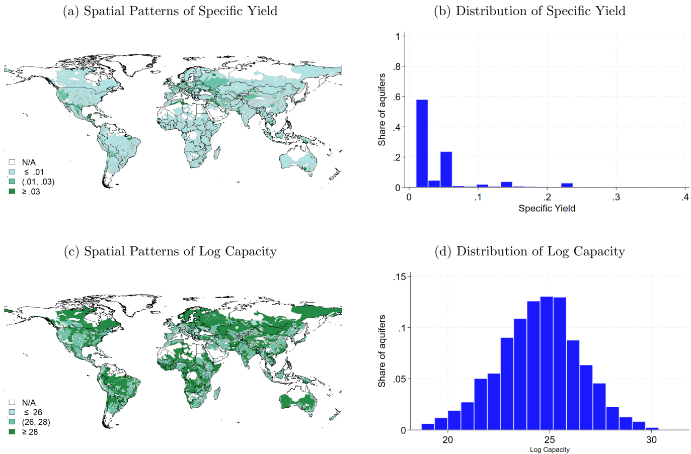
Figure A.1: Patterns of Specific Yield and Capacity, by Aquifer
