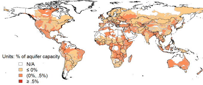
(c) Spatial Patterns of Annual Recharge
