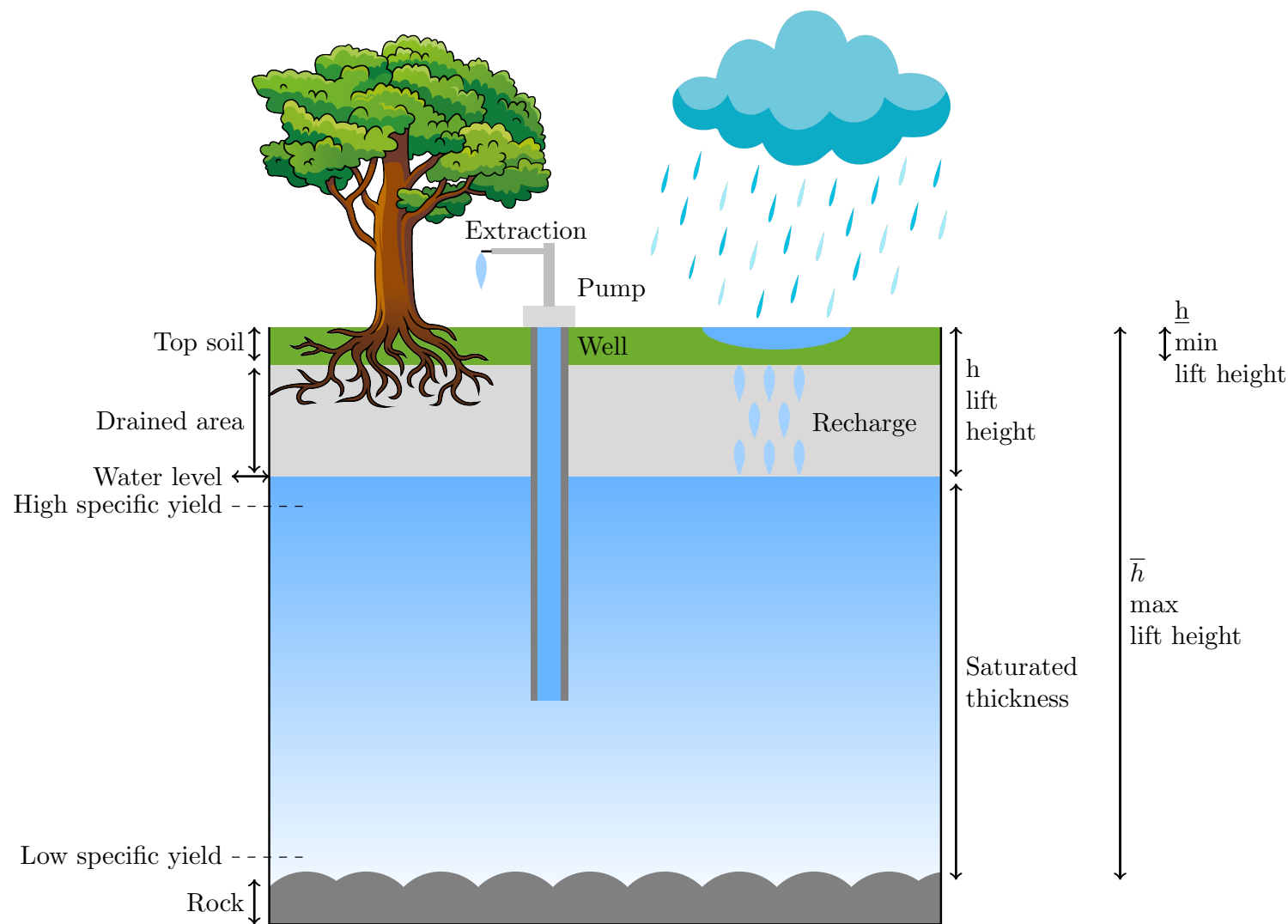
Figure 1: Aquifer Structure and Terminology
